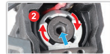
Use 8mm Allen key to depress the spring guide and rotate 45°, carefully and slowly remove the guide.
