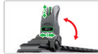
● Flip up or fold down. ● Elevation knob (up / down adjustment).
